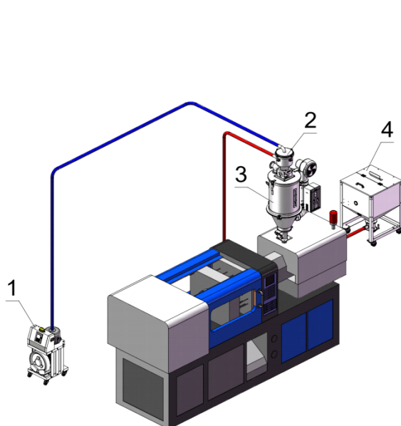
FAL-2P application
